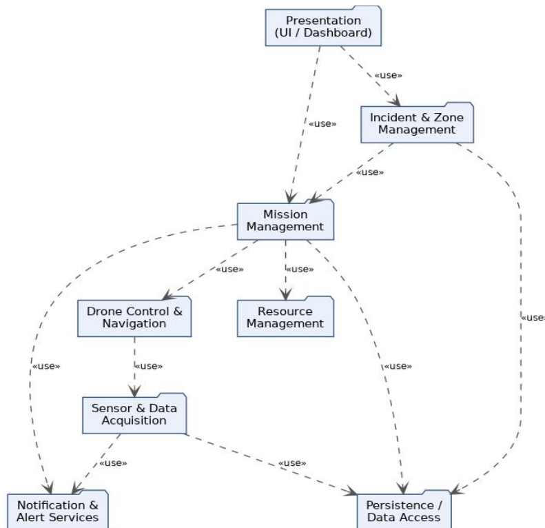
Figure 10.1 — Package Diagram for ADDRRS
