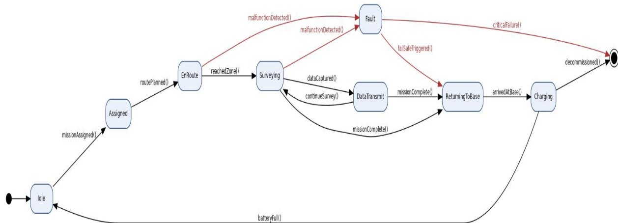
Figure 9.1 — State Transition Diagram for the Drone Class
