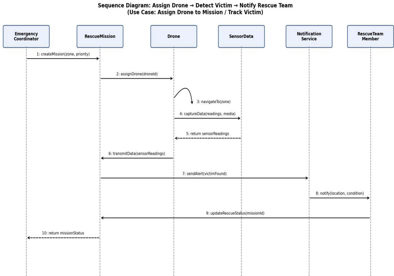
Figure 7.1 — Sequence Diagram: Assign Drone → Detect Victim → Notify Rescue Team
