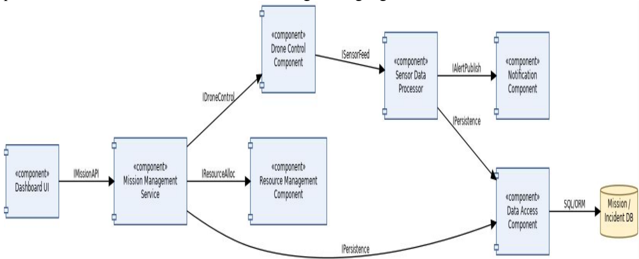
Figure 11.1 — Component Diagram for ADDRRS
