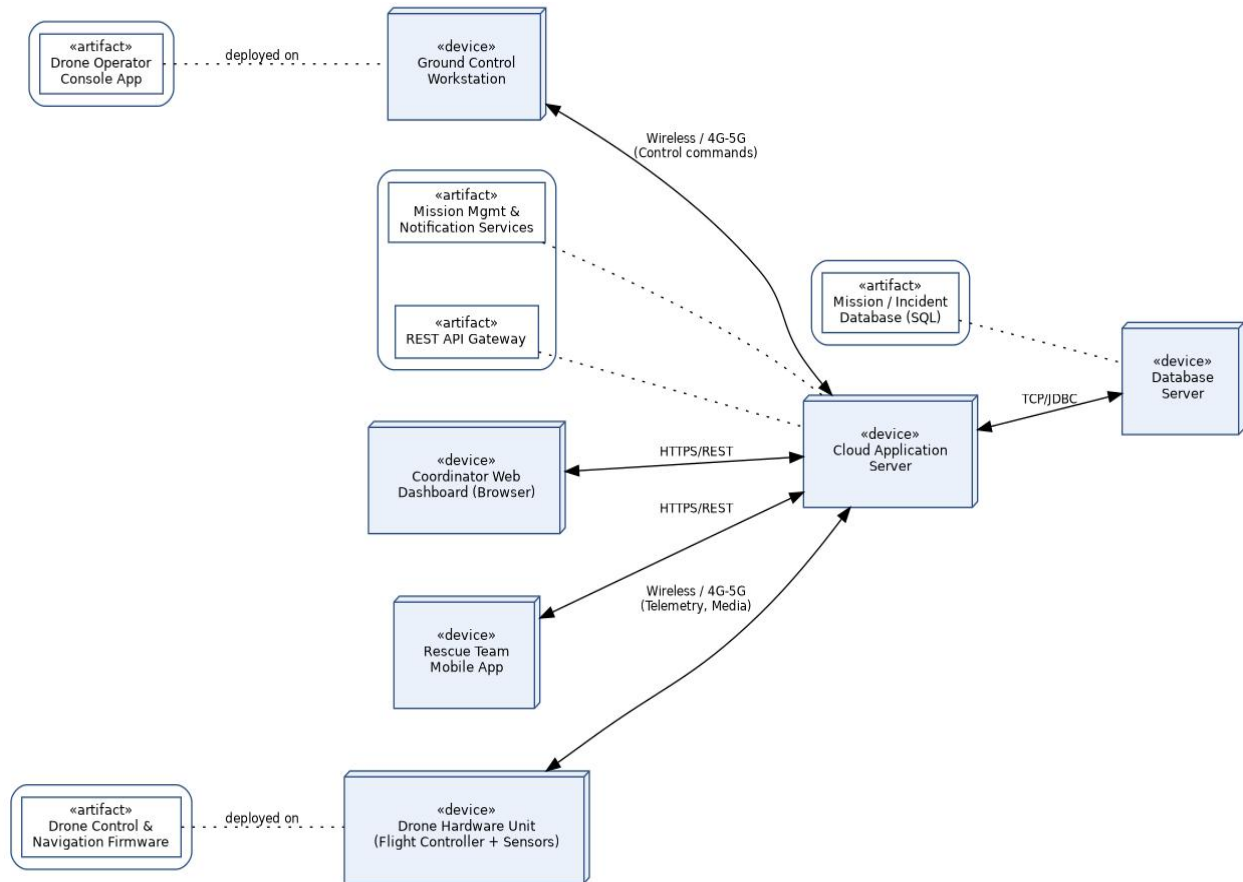
Figure 12.1 — Deployment Diagram for ADDRRS
