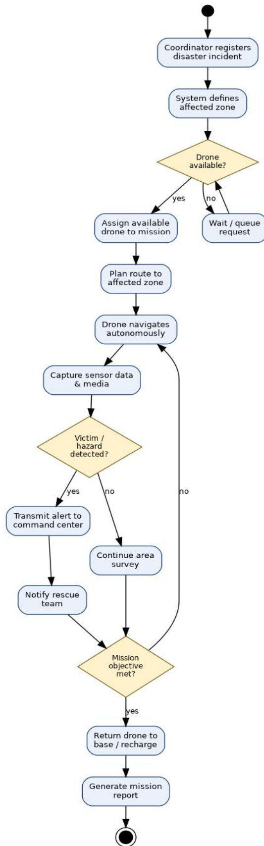
Figure 8.1 — Activity Diagram: End-to-End Rescue Mission Workflow
