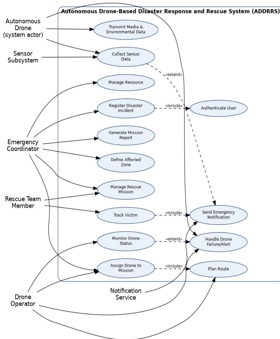
Figure 4.1 — Use Case Diagram for ADDRRS
